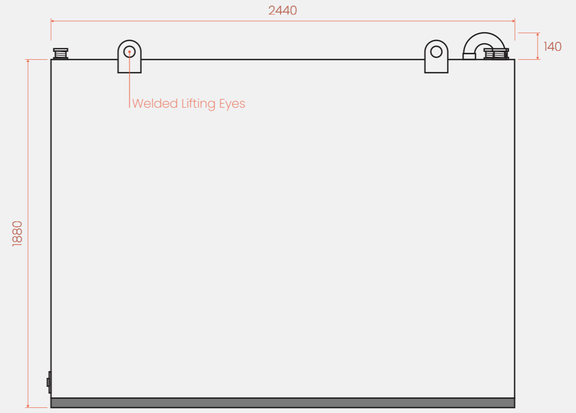
Right
