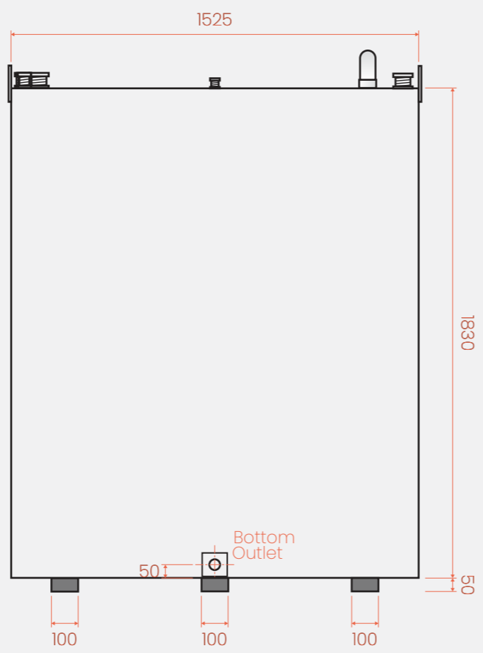
Front
